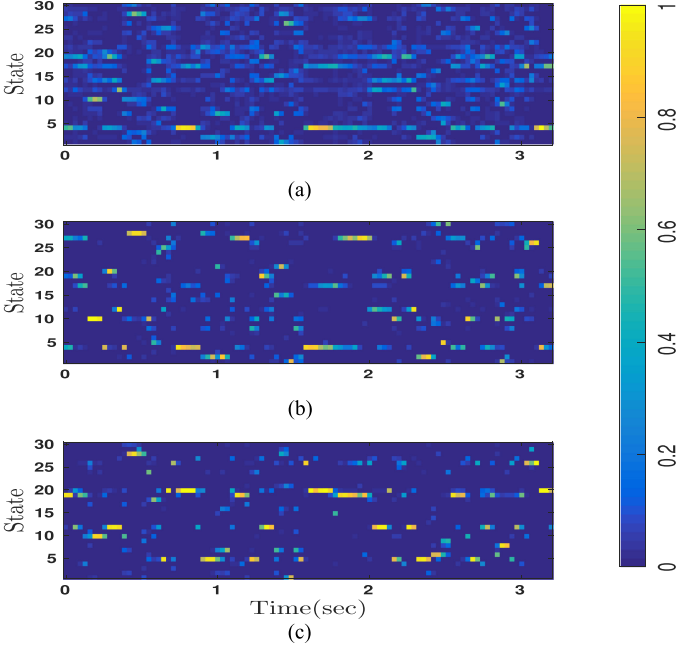
Fig. 10. Compactness of representation indicated by state activation in (a) PLCA, (b) DLVM, and (c) bi-DLVM.
