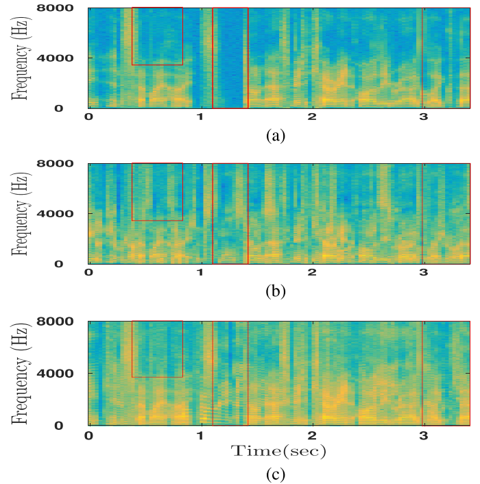
Fig. 4. Sample result for speaker source separation: (a) original source, (b) recovered source using PLCA, (c) recovered source using DLVM.
