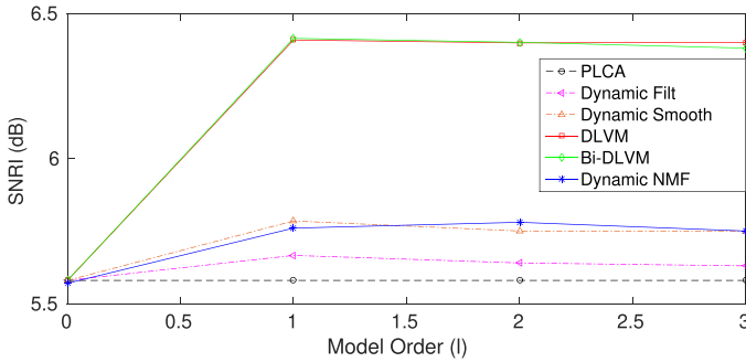
Fig. 6. Source separation performance with varying model order.
