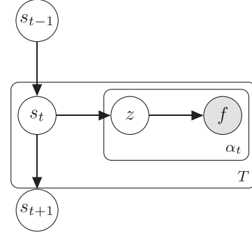
Fig. 1. Plate notation for DLVM ( T : total number of time instants).
