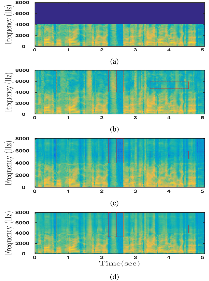
Fig. 9. Sample result for bandwidth expansion: (a) bandlimited signal, (b) original signal, (c) bandwidth expansion using PLCA, and (d) bandwidth expansion using DLVM.
