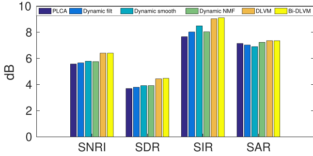
Fig. 5. Performance comparison for speaker source separation in terms of four evaluation metrics.
