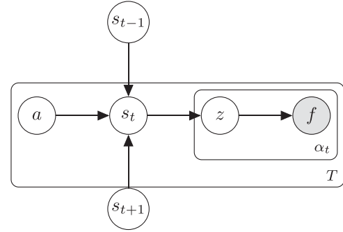
Fig. 3. Plate notation of the mixture signal modeled using bi-DLVM, a denotes an audio source.
