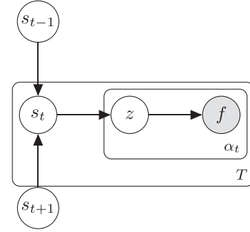
Fig. 2. Plate notation for bi-DLVM (order = 1).
