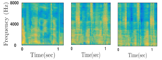
Fig. 7. Sample denoising result: (left) original source (left), (center) source recovered by PLCA, and (right) DLVM at 6 dB SNR.
